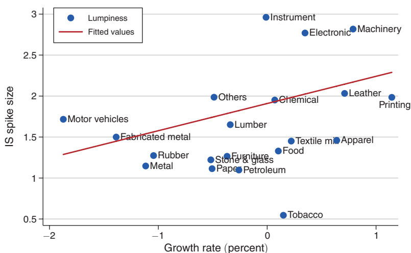
FIGURE 13. IS SPIKES AND \bar{g}
