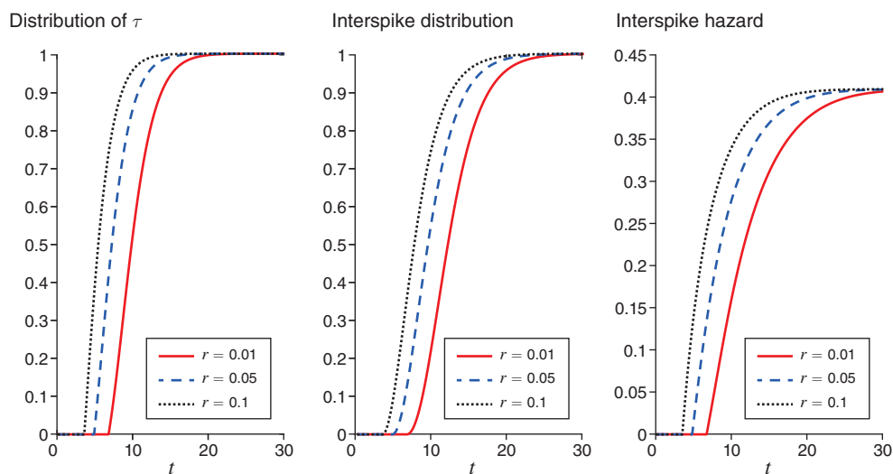
FIGURE 5. THE EFFECT OF r AT \lambda_L = 1, \lambda_H = 0.4, g = 0.1
