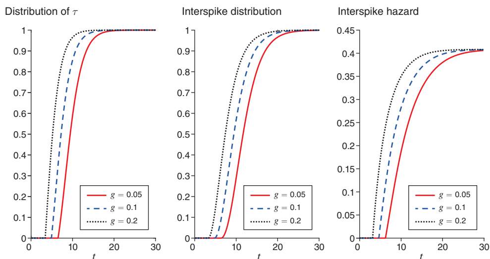
FIGURE 3. THE EFFECT OF g AT \lambda_L = 1, \lambda_H = 0.4, r = 0.05
