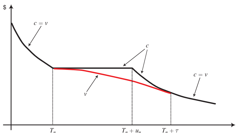
FIGURE 1. c_t > v_t ON THE INTERVAL (0, \tau)
