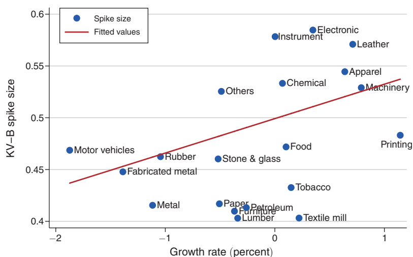
FIGURE 15. KV-B SPIKES AND \bar{g}
