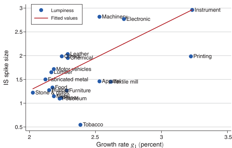
FIGURE 7. IS SPIKES AND \hat{g}_1
