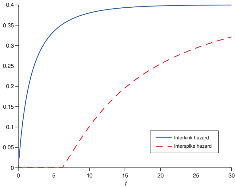
FIGURE 2. \eta(t) (SOLID) AND H'/(1-H) (DASHED) AT \lambda_L = 0.6 , \lambda_H = 0.4 , r = 0.05 , AND g = 0.1
