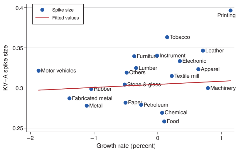
FIGURE 14. KV-A SPIKES AND \bar{g}
