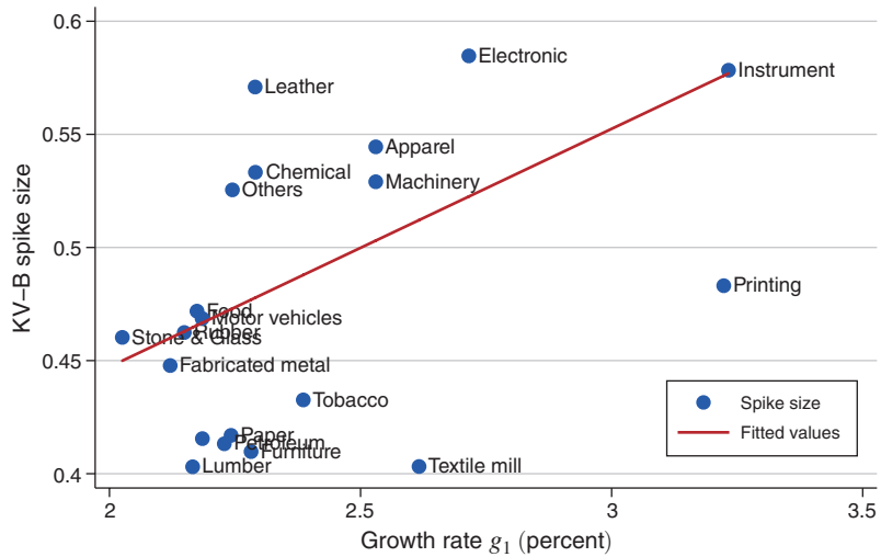
FIGURE 9. KV-B SPIKES AND \hat{g}_1
