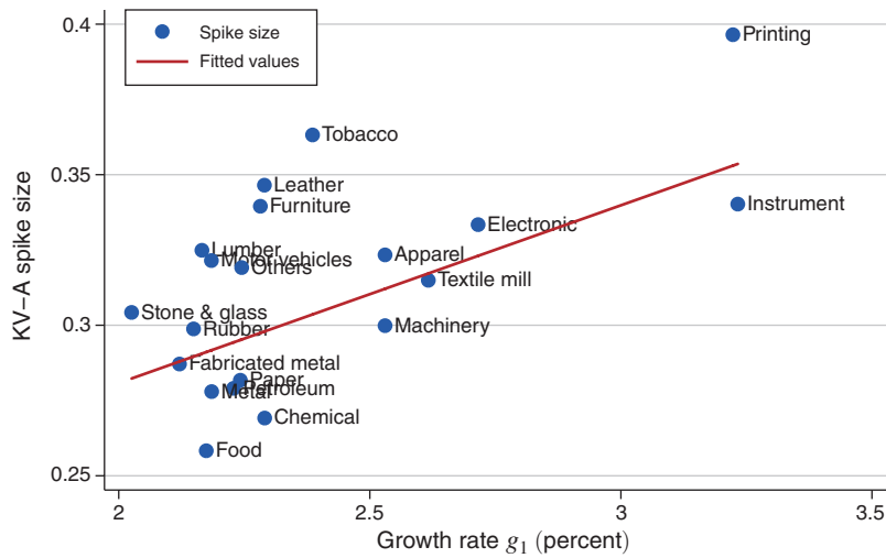
FIGURE 8. KV-A SPIKES AND \hat{g}_1
