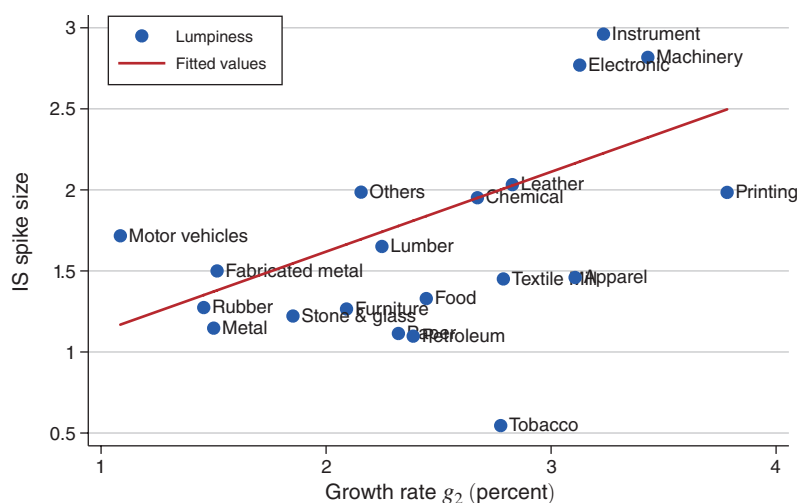
FIGURE 10. IS SPIKES AND \hat{g}_2
