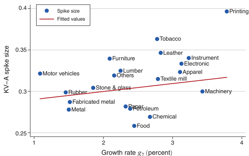
FIGURE 11. KV-A SPIKES AND \hat{g}_2
