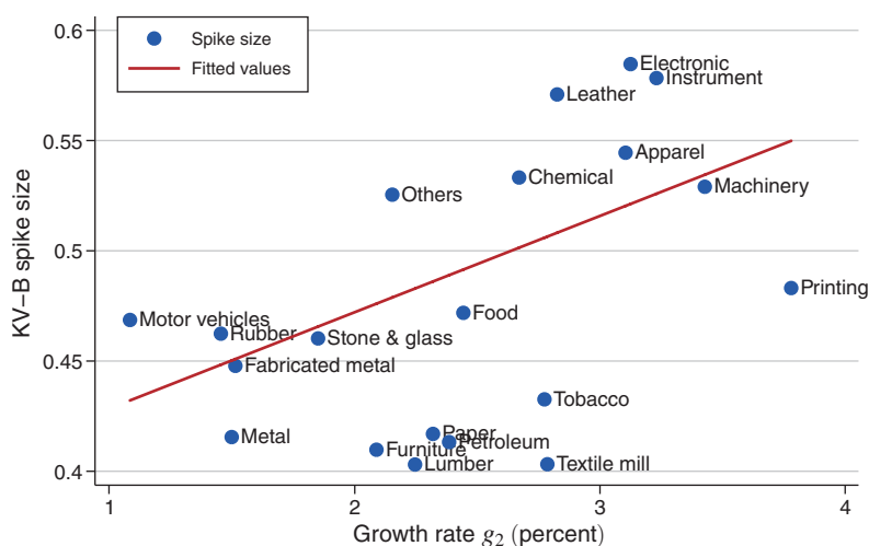
FIGURE 12. KV-B SPIKES AND \hat{g}_2
