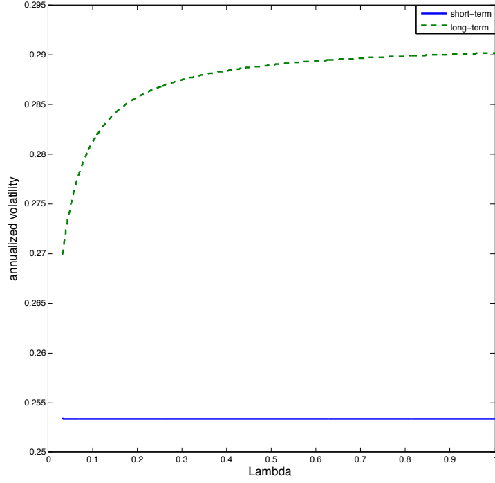
Figure 2: Volatility of basic securities and primary market liquidity, \Lambda_C . Short- and long-term volatilities are defined as square roots of expressions in (63), but annualized: the short-term volatility is multiplied by 252^{1/2} , the long-term one is multiplied by (252/2)^{1/2} . Parameter values: N = 10 ; L = 1 ; \Sigma_d = \text{Id} + \mathbf{1}_{N \times N} ; \Sigma_\varepsilon = \Sigma_\xi = 0.05 \text{Id} , \alpha_* = 0.2 , \alpha_{*E} = 0.2 ; \alpha_{*D} = 0.02 ; r = 0.05/252 ; \mathbf{F} = \frac{1}{N}\mathbf{1} .
