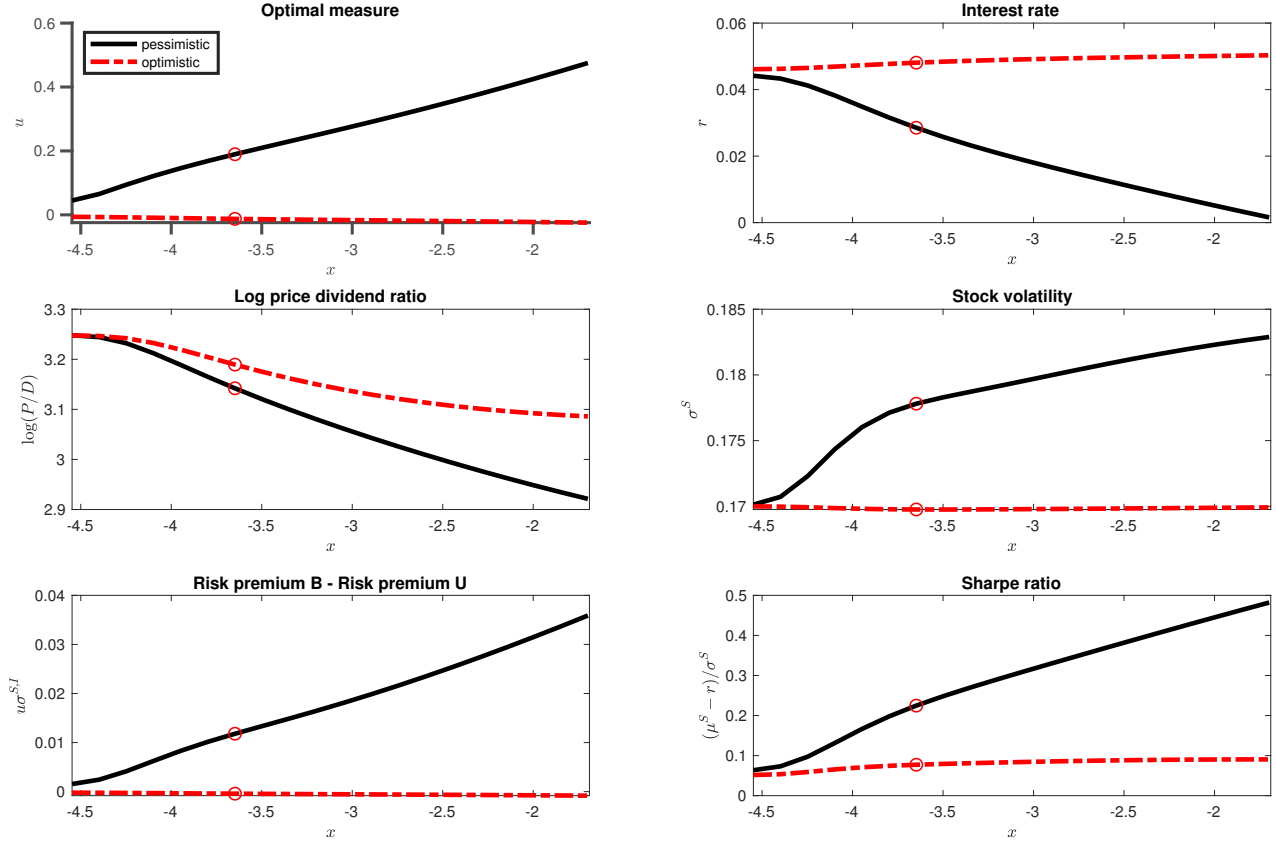
Figure 5. General equilibrium quantities
