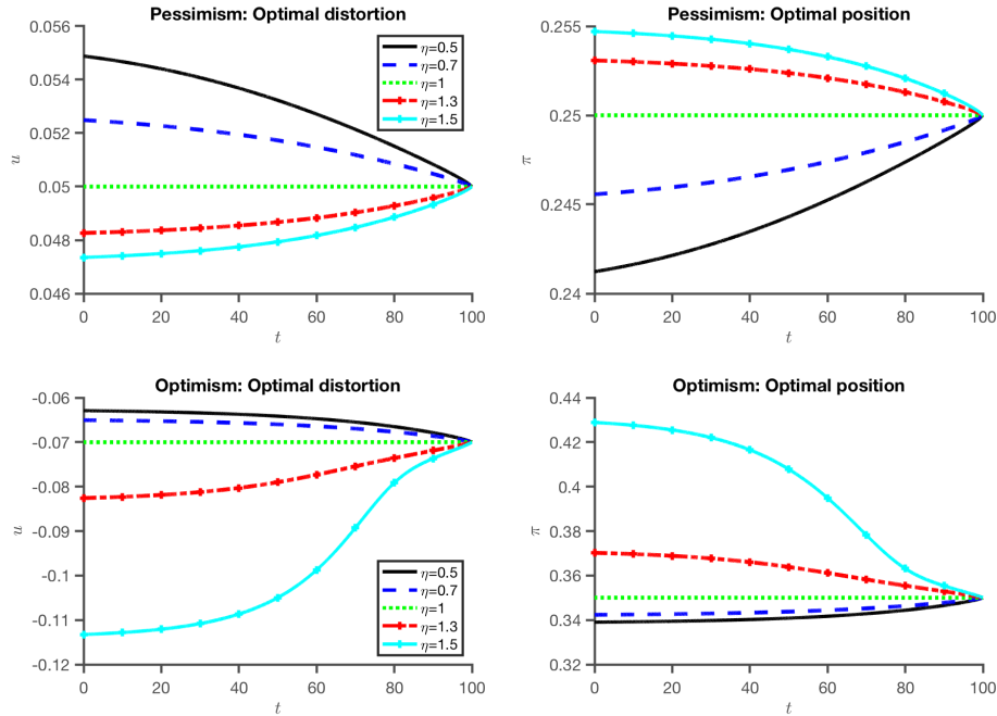
Figure 3. Time dependence of optimal distortions and portfolios
