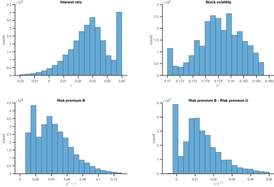
Figure 6. Distribution of equilibrium quantities
