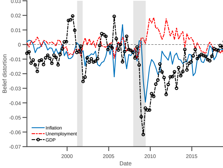
Figure 1. Belief Distortions: Difference between Subjective and Objective Beliefs
