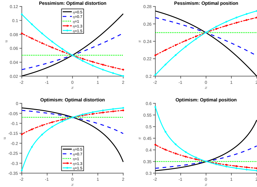
Figure 2. State dependent optimal distortions and portfolios
