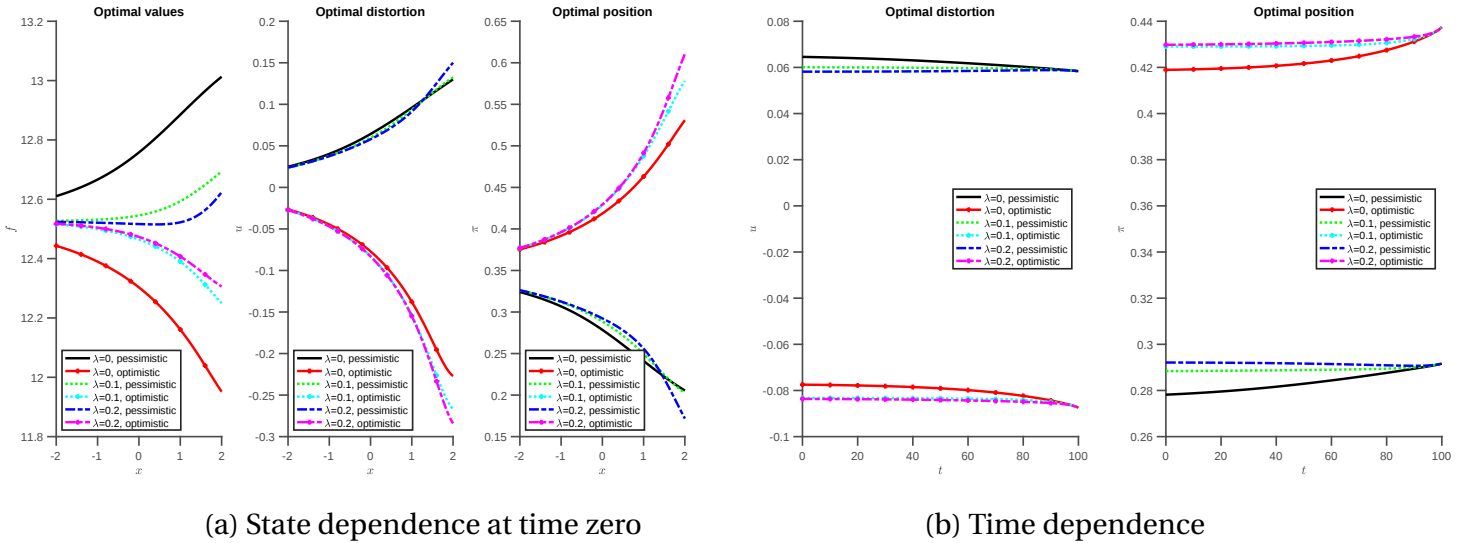
Figure 4. Value functions, optimal distortions and portfolios in regime switching models
